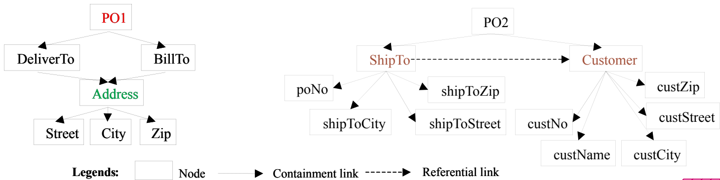
Graph representation of schemas (COMA++)
