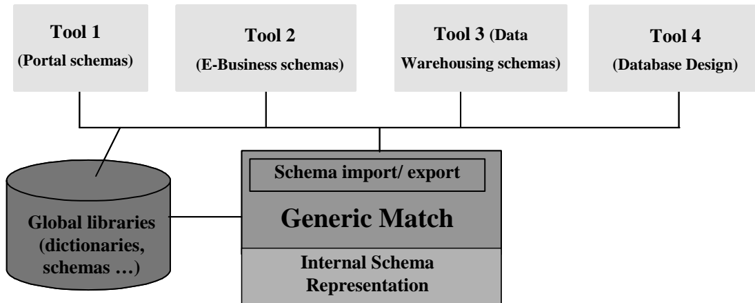
Figure 1: High Level Architecture of Generic Match
