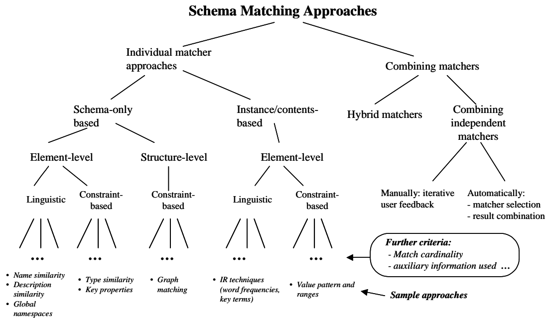
Figure 2: Classification of schema matching approaches
