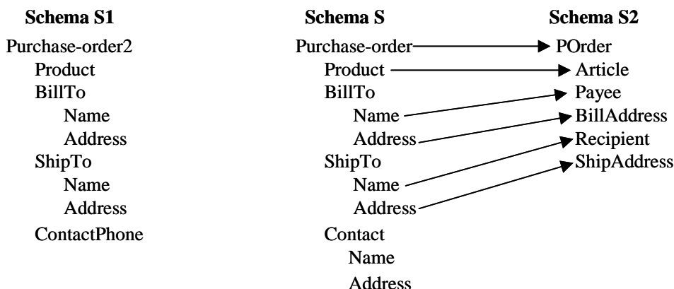
Figure 4: Scenario for reuse of an existing Match mapping
